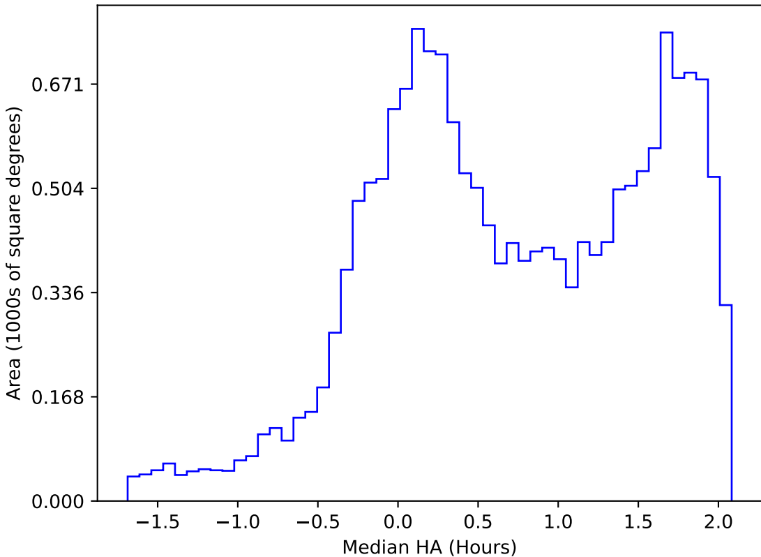
internal_u_expt45_nscale1.2v3.4_10yrs WFD g band: Median HA
