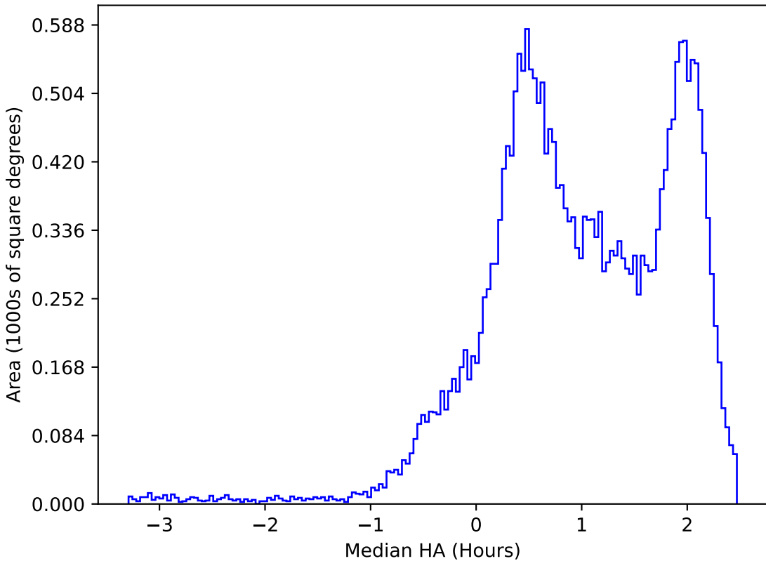
internal_u_expt45_nscale1.2v3.4_10yrs All sky z band: Median HA
