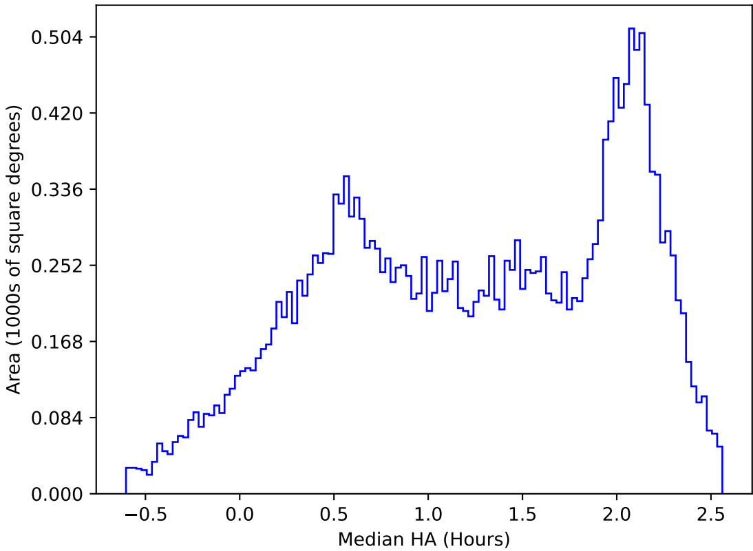
internal_u_expt45_nscale1.2v3.4_10yrs All sky y band: Median HA
