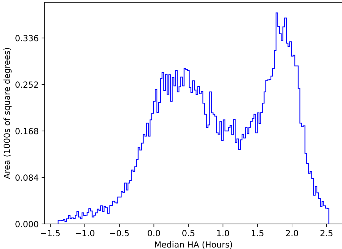
internal_u_expt45_nscale1.2v3.4_10yrs All sky u band: Median HA
