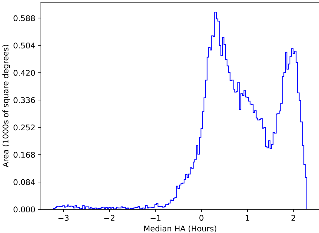
internal_u_expt45_nscale1.2v3.4_10yrs All sky i band: Median HA
