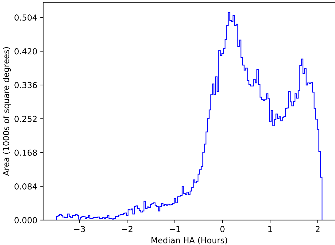
internal_u_expt45_nscale1.2v3.4_10yrs All sky g band: Median HA
