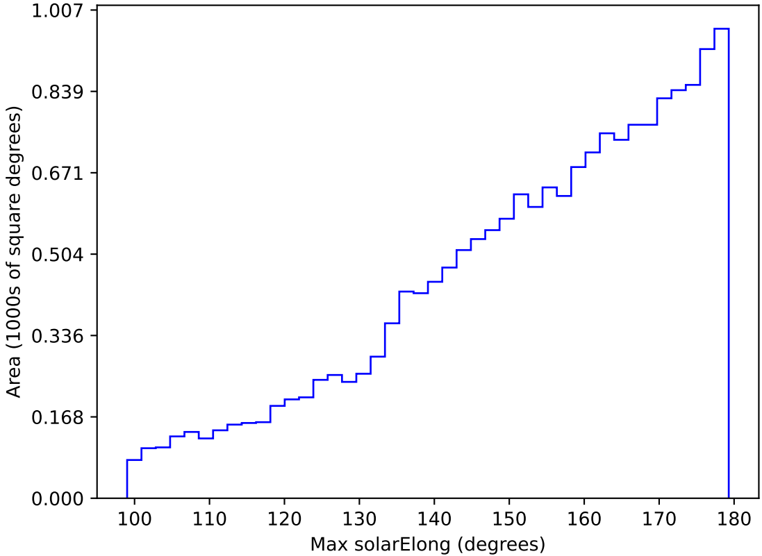
internal_u_expt45_nscale1.2v3.4_10yrs WFD y band: Max solarElong
