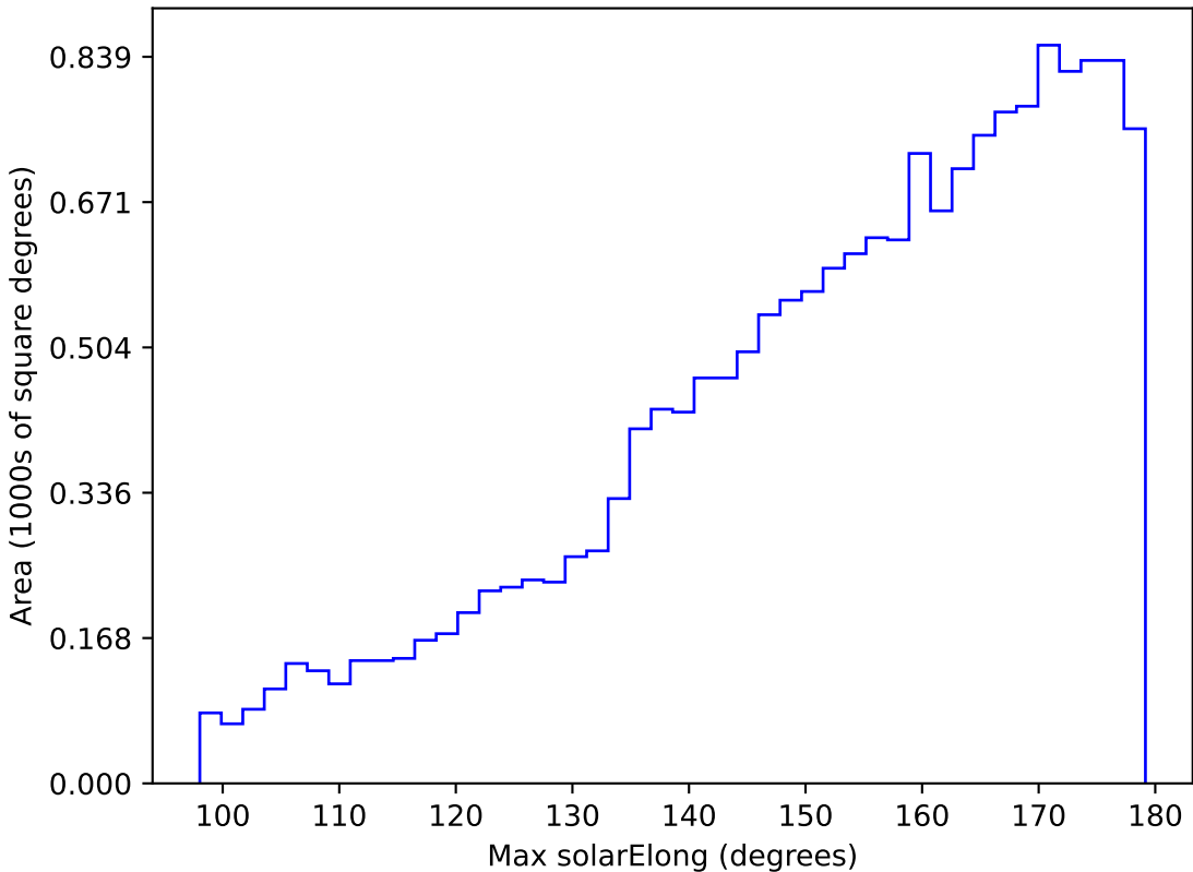
internal_u_expt45_nscale1.2v3.4_10yrs WFD u band: Max solarElong
