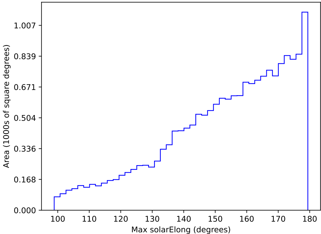
internal_u_expt45_nscale1.2v3.4_10yrs WFD r band: Max solarElong
