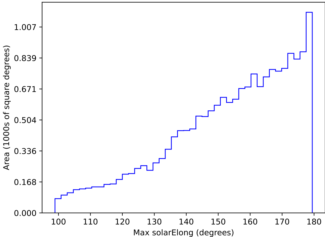
internal_u_expt45_nscale1.2v3.4_10yrs WFD i band: Max solarElong
