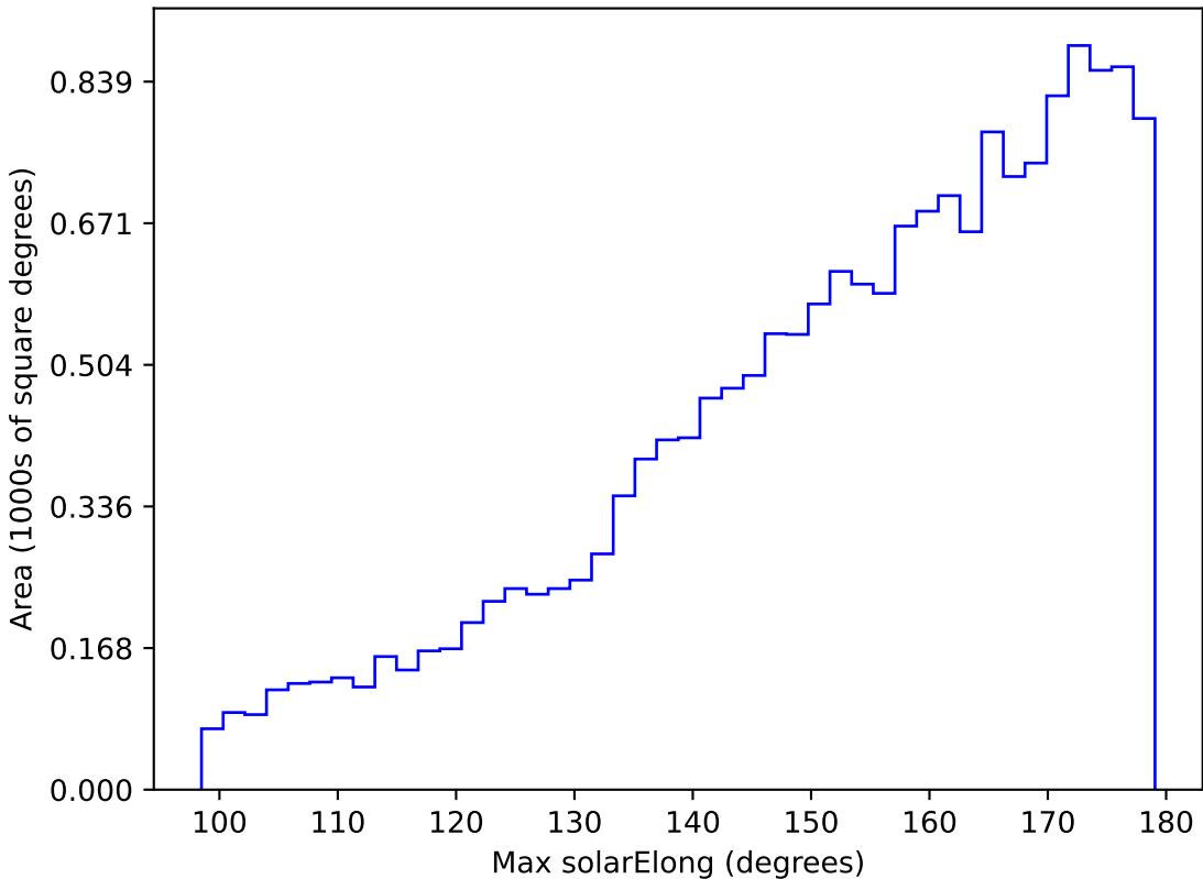
internal_u_expt45_nscale1.2v3.4_10yrs WFD g band: Max solarElong
