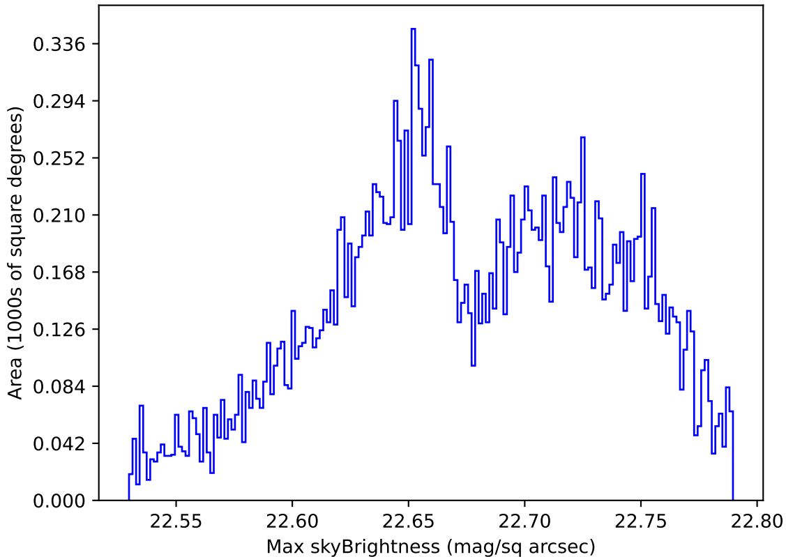
internal_u_expt45_nscale1.2v3.4_10yrs Yr 1 u band: Max skyBrightness
