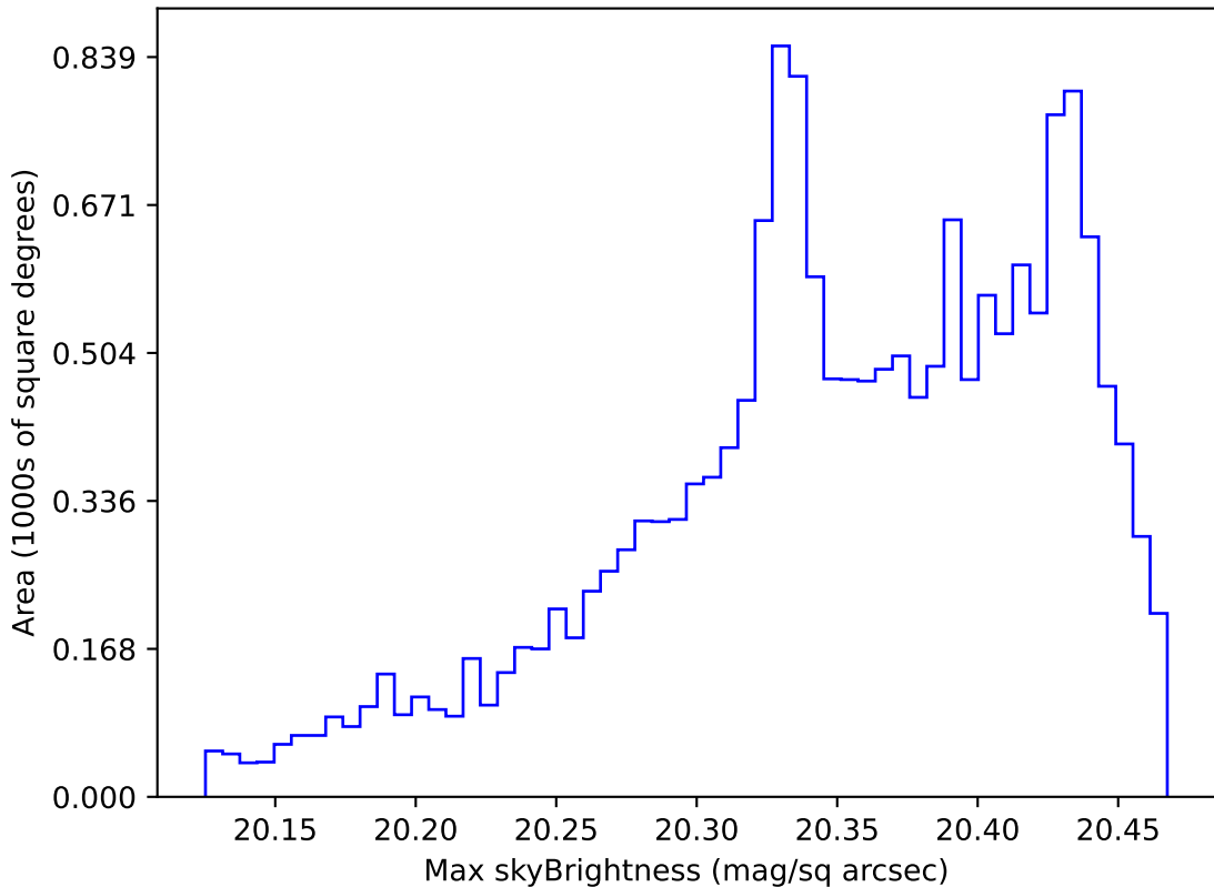
internal_u_expt45_nscale1.2v3.4_10yrs WFD i band: Max skyBrightness
