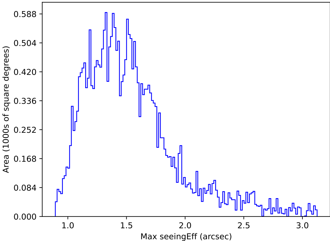
internal_u_expt45_nscale1.2v3.4_10yrs Yr 1 i band: Max seeingEff
