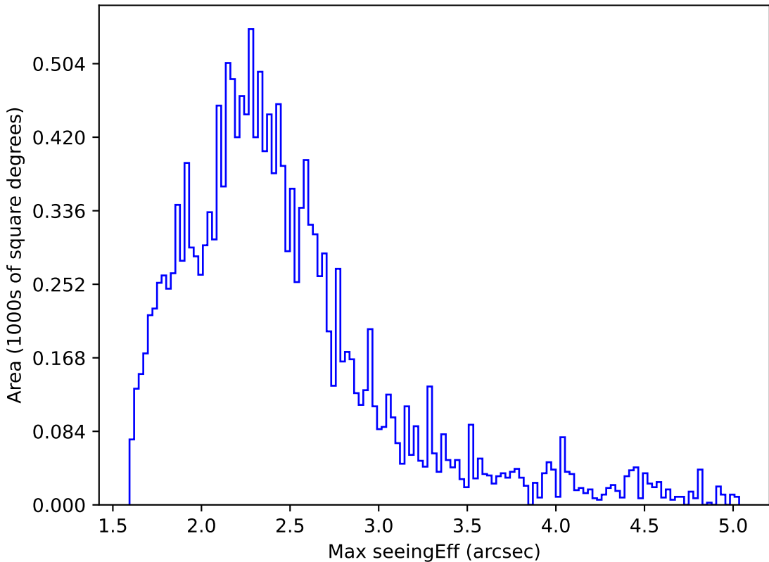
internal_u_expt45_nscale1.2v3.4_10yrs WFD y band: Max seeingEff
