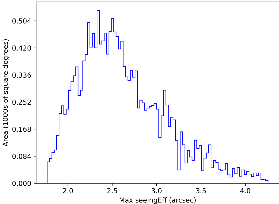
internal_u_expt45_nscale1.2v3.4_10yrs WFD u band: Max seeingEff
