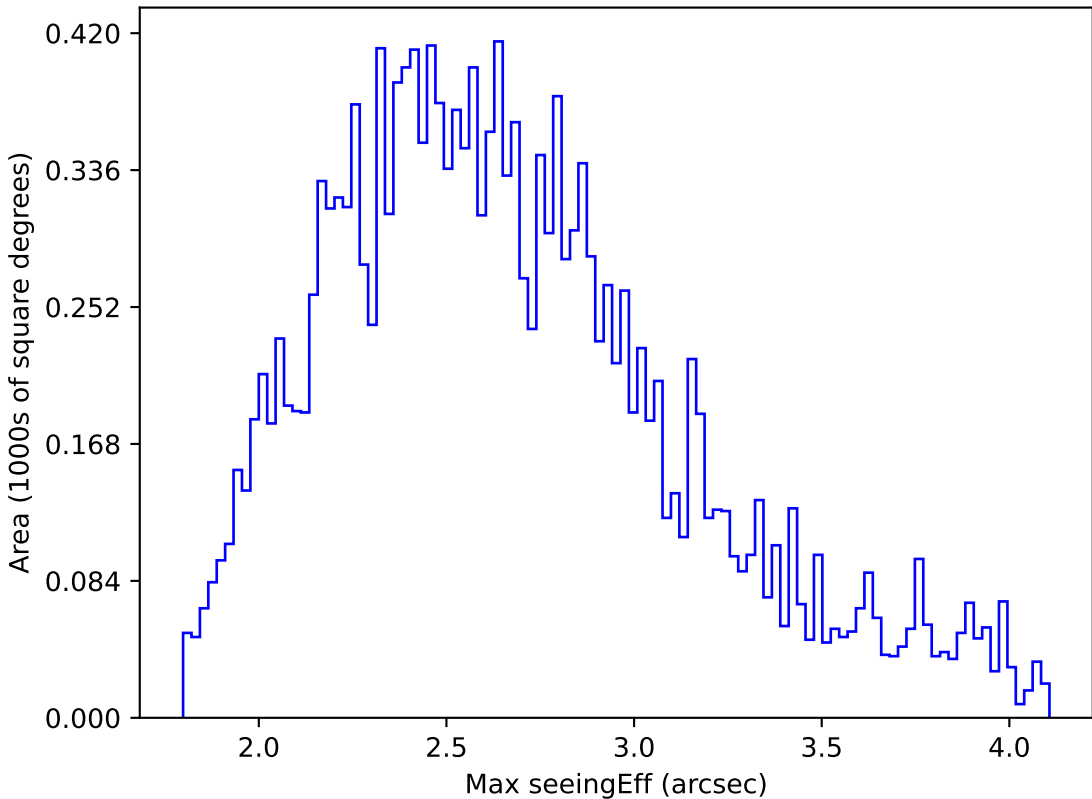
internal_u_expt45_nscale1.2v3.4_10yrs WFD r band: Max seeingEff
