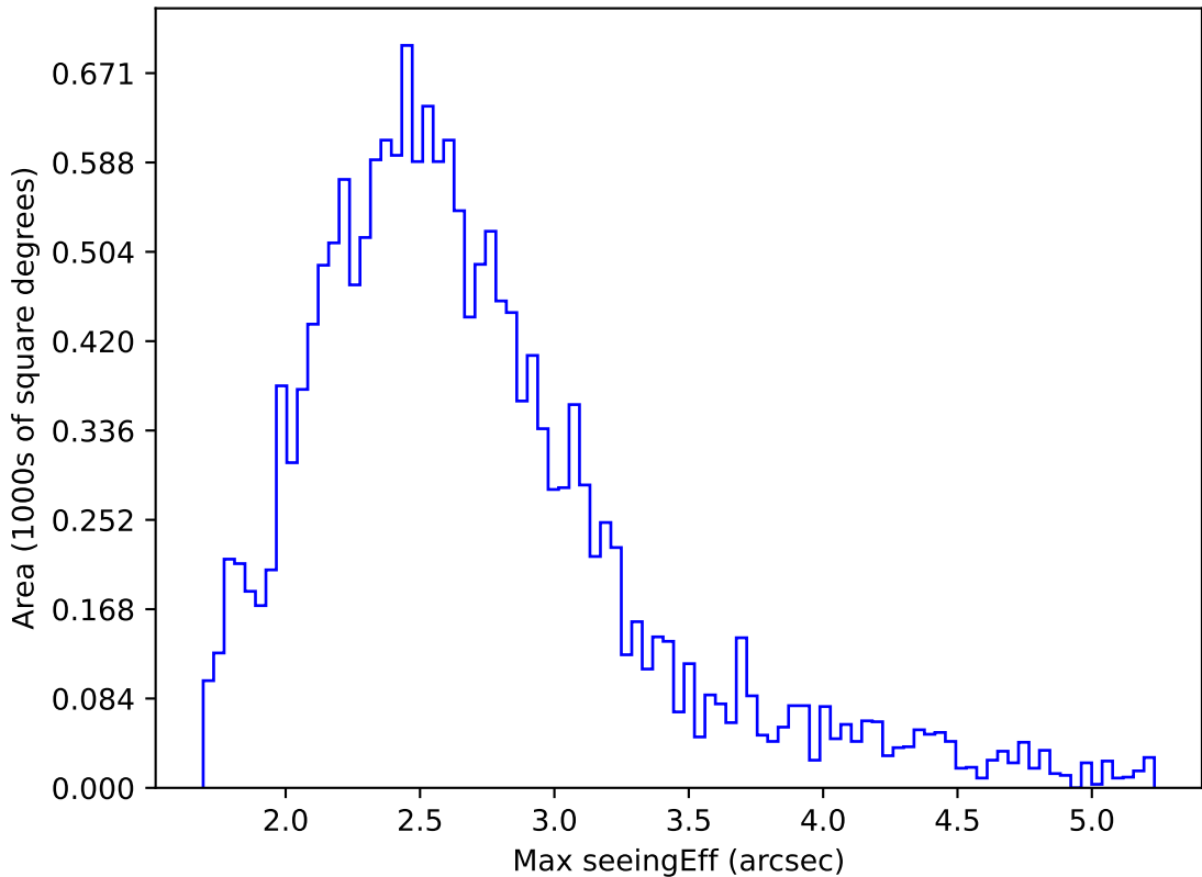
internal_u_expt45_nscale1.2v3.4_10yrs WFD i band: Max seeingEff
