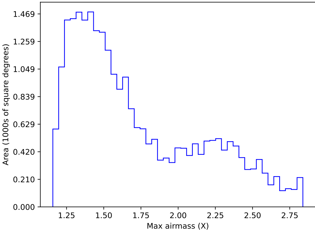
internal_u_expt45_nscale1.2v3.4_10yrs Yr 1 z band: Max airmass
