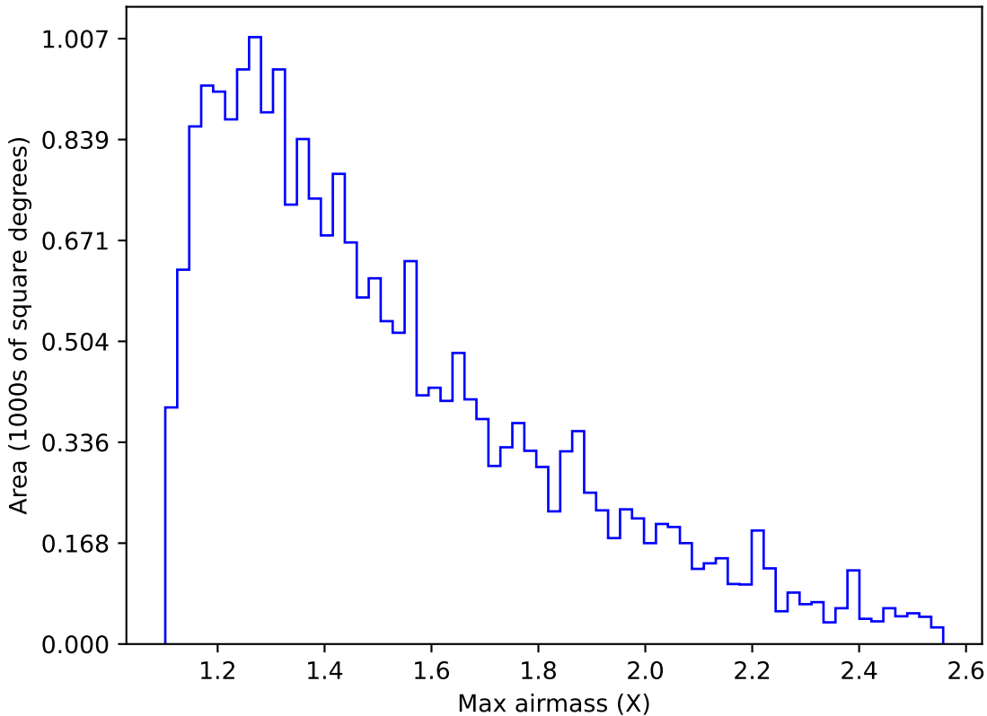
internal_u_expt45_nscale1.2v3.4_10yrs Yr 1 u band: Max airmass
