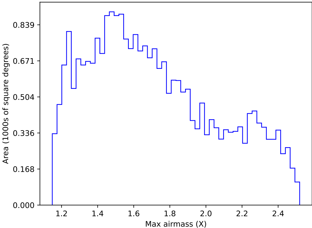
internal_u_expt45_nscale1.2v3.4_10yrs Yr 1 r band: Max airmass
