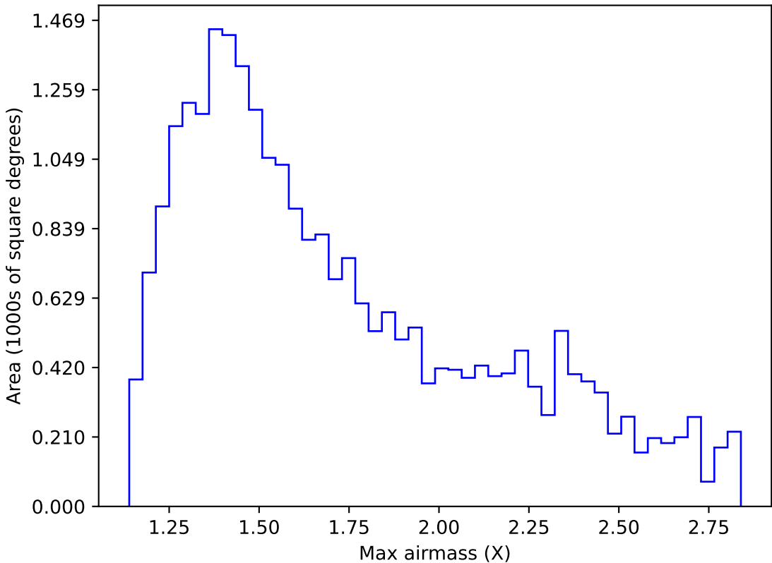
internal_u_expt45_nscale1.2v3.4_10yrs Yr 1 i band: Max airmass
