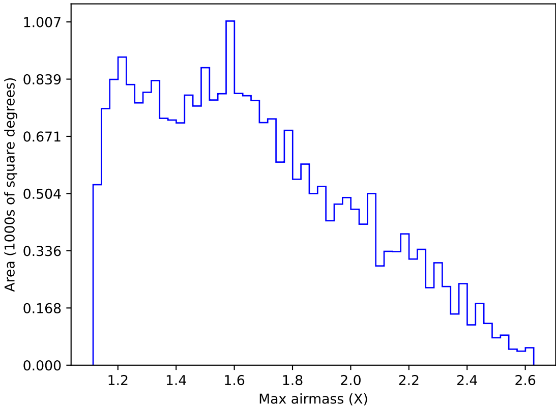
internal_u_expt45_nscale1.2v3.4_10yrs Yr 1 g band: Max airmass
