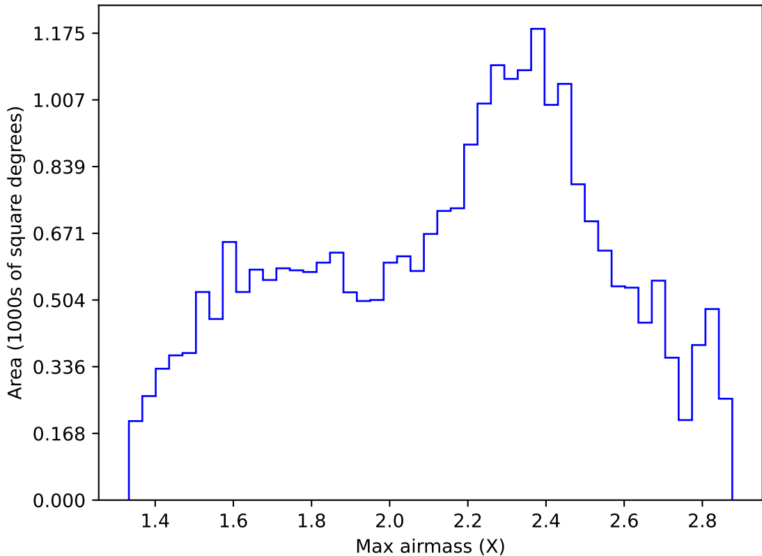
internal_u_expt45_nscale1.2v3.4_10yrs Yr 1 all bands: Max airmass
