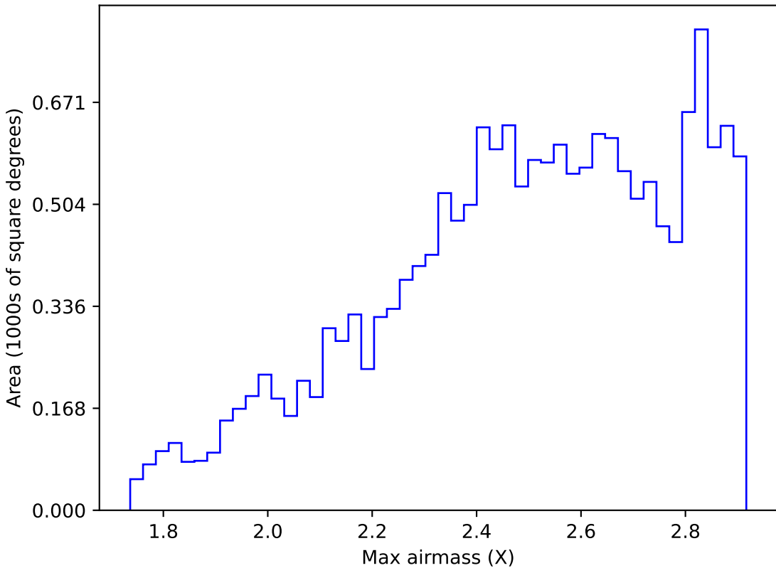
internal_u_expt45_nscale1.2v3.4_10yrs WFD z band: Max airmass
