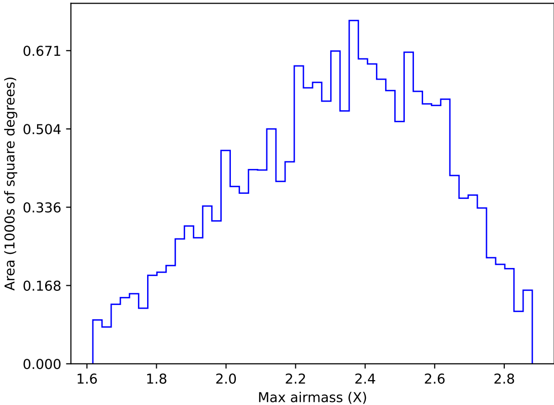
internal_u_expt45_nscale1.2v3.4_10yrs WFD y band: Max airmass
