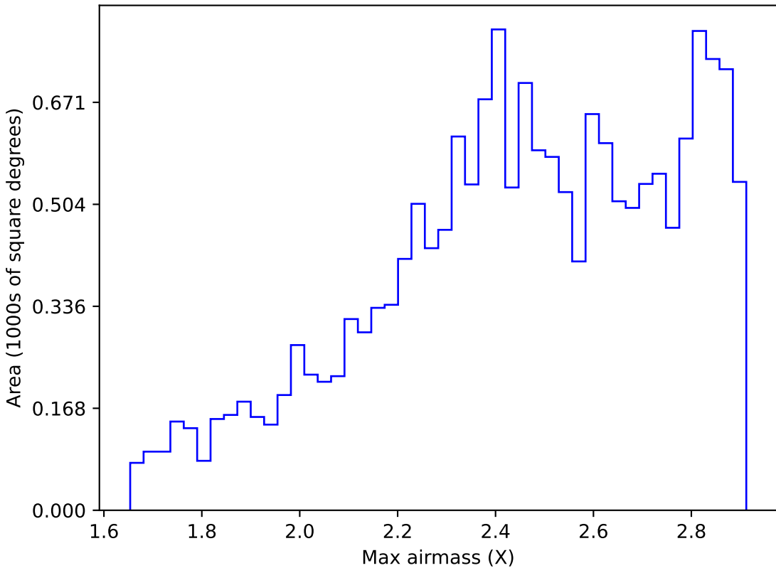
internal_u_expt45_nscale1.2v3.4_10yrs WFD i band: Max airmass
