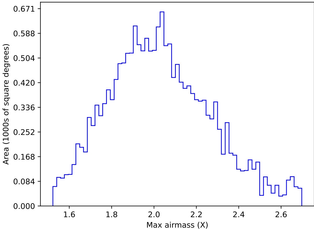
internal_u_expt45_nscale1.2v3.4_10yrs WFD g band: Max airmass
