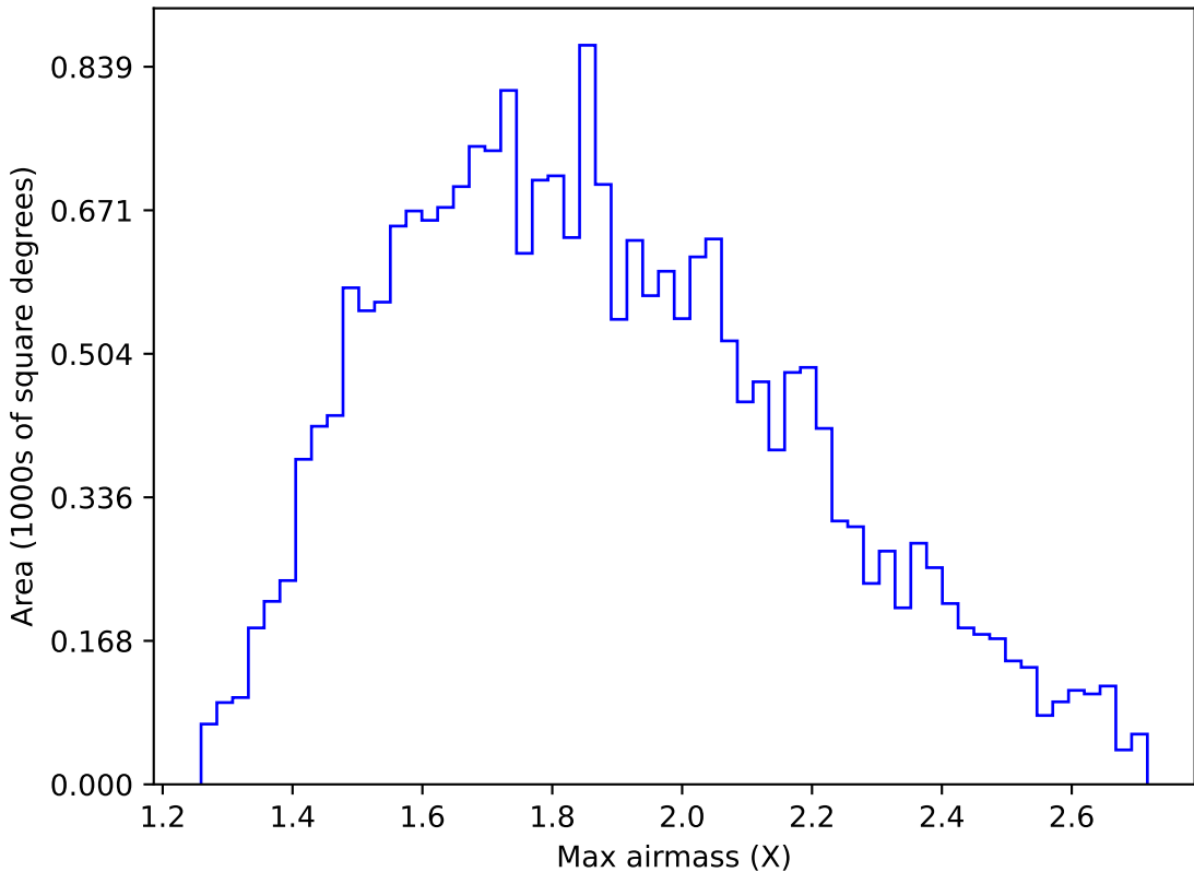
internal_u_expt45_nscale1.2v3.4_10yrs All sky u band: Max airmass
