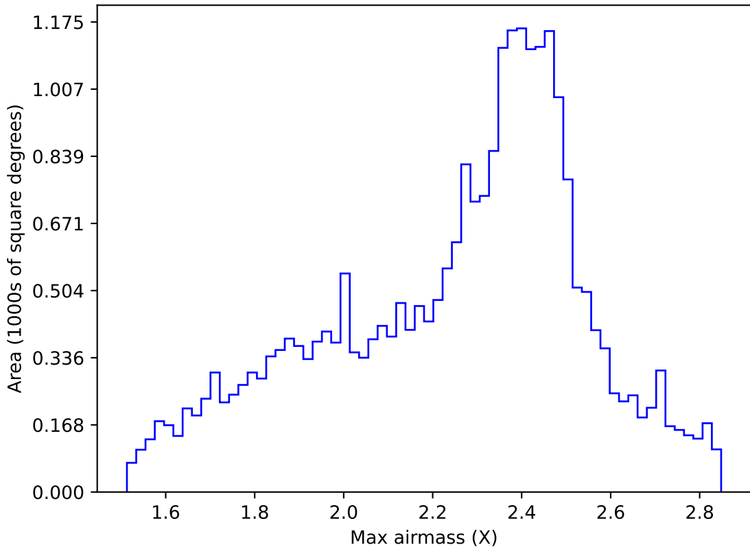
internal_u_expt45_nscale1.2v3.4_10yrs All sky r band: Max airmass
