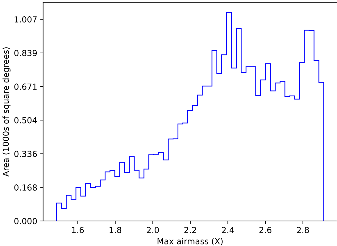
internal_u_expt45_nscale1.2v3.4_10yrs All sky i band: Max airmass
