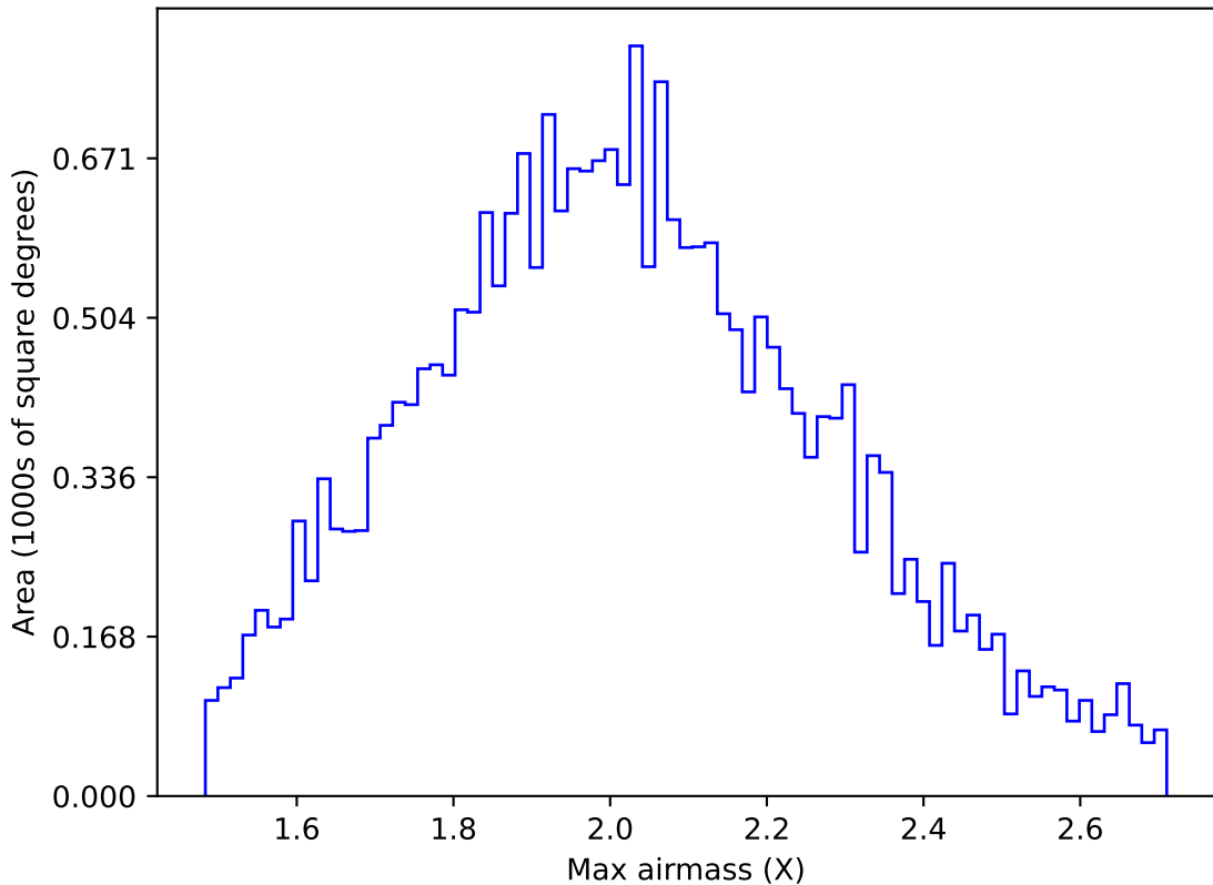
internal_u_expt45_nscale1.2v3.4_10yrs All sky g band: Max airmass
