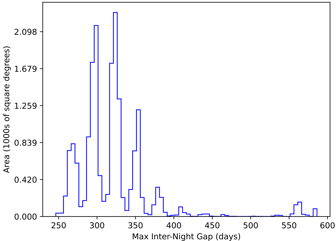
internal_u_expt45_nscale1.2v3.4_10yrs WFD y band: Max Inter-Night Gap
