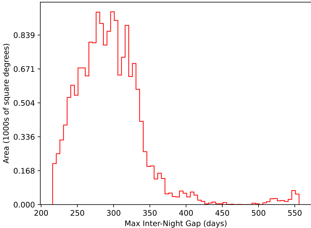
internal_u_expt45_nscale1.2v3.4_10yrs WFD i band: Max Inter-Night Gap
