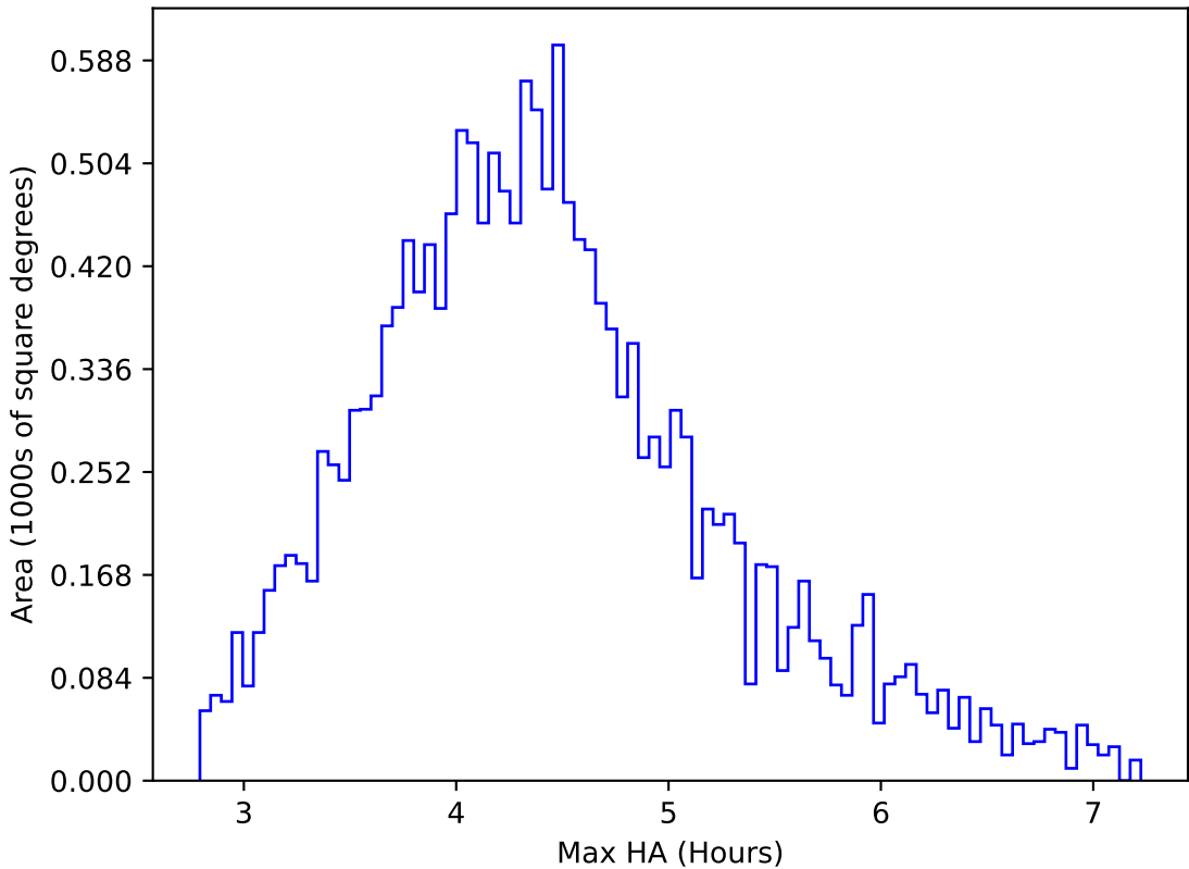
internal_u_expt45_nscale1.2v3.4_10yrs WFD r band: Max HA
