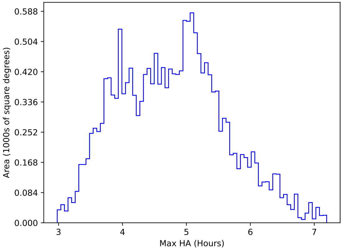
internal_u_expt45_nscale1.2v3.4_10yrs WFD i band: Max HA
