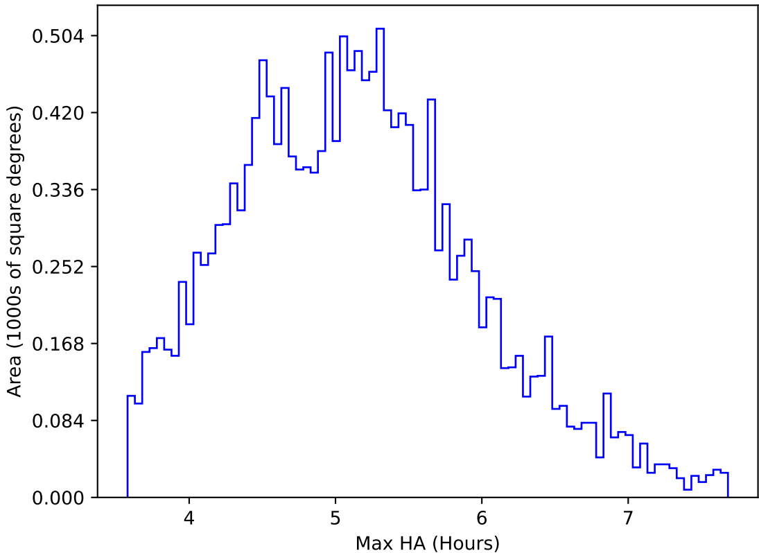
internal_u_expt45_nscale1.2v3.4_10yrs WFD all bands: Max HA
