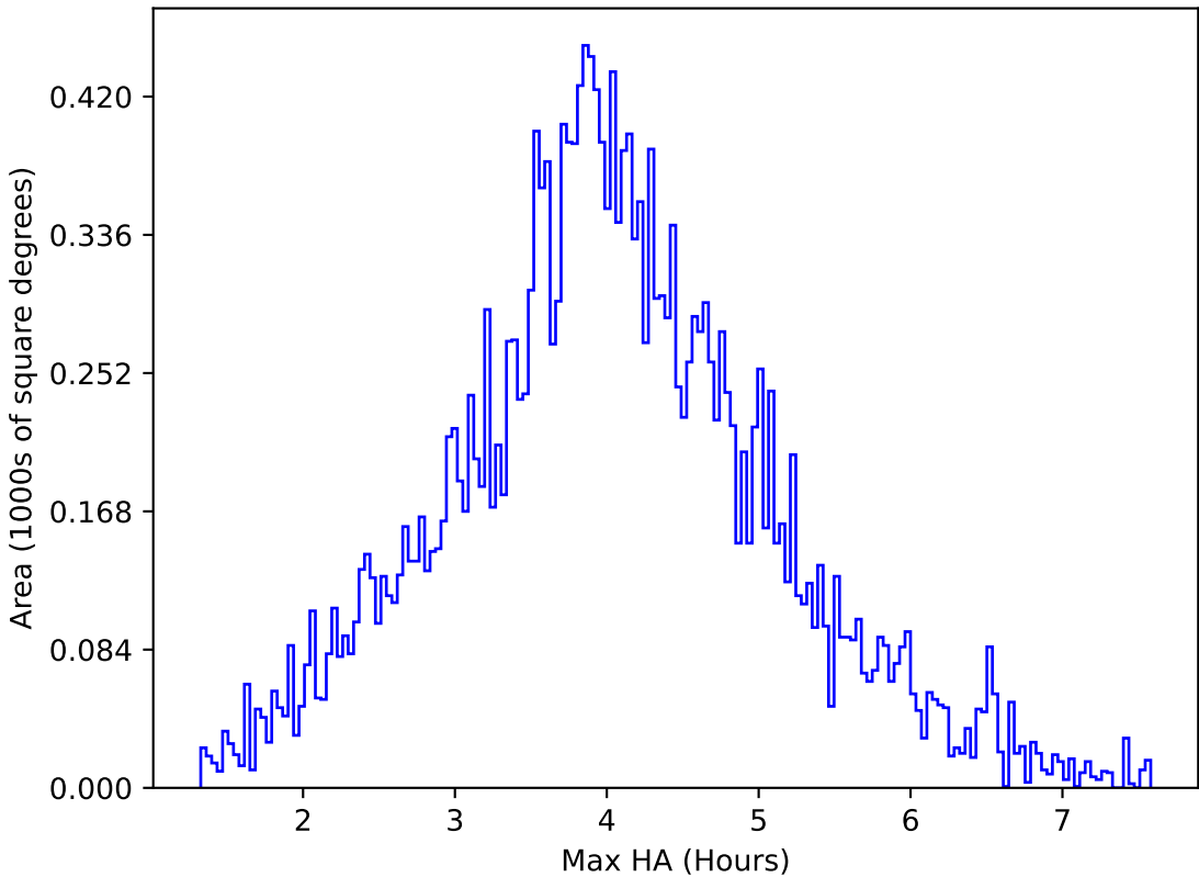
internal_u_expt45_nscale1.2v3.4_10yrs All sky u band: Max HA
