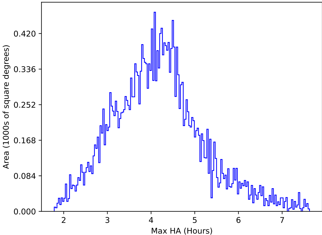
internal_u_expt45_nscale1.2v3.4_10yrs All sky r band: Max HA
