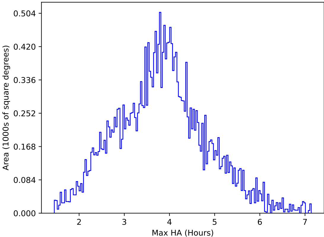
internal_u_expt45_nscale1.2v3.4_10yrs All sky g band: Max HA
