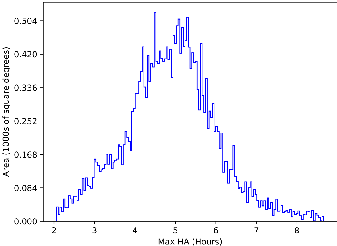
internal_u_expt45_nscale1.2v3.4_10yrs All sky all bands: Max HA
