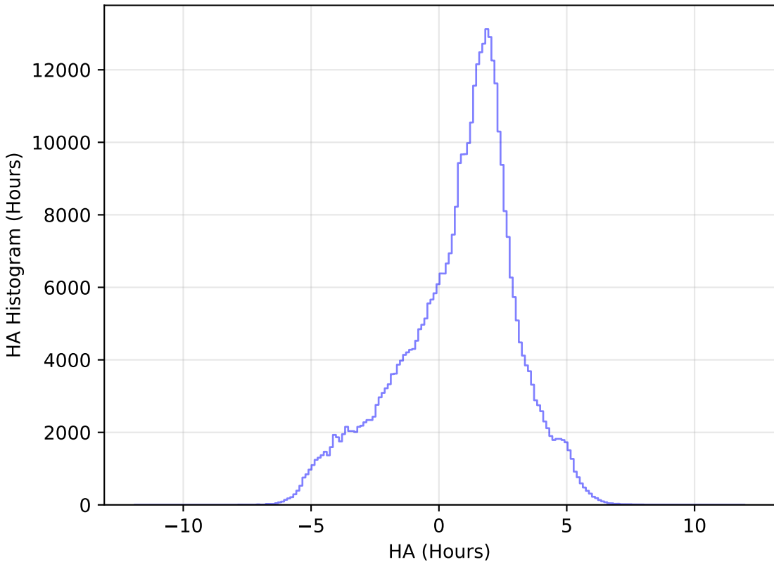
internal_u_expt45_nscale1.2v3.4_10yrs WFD z band: HA Histogram
