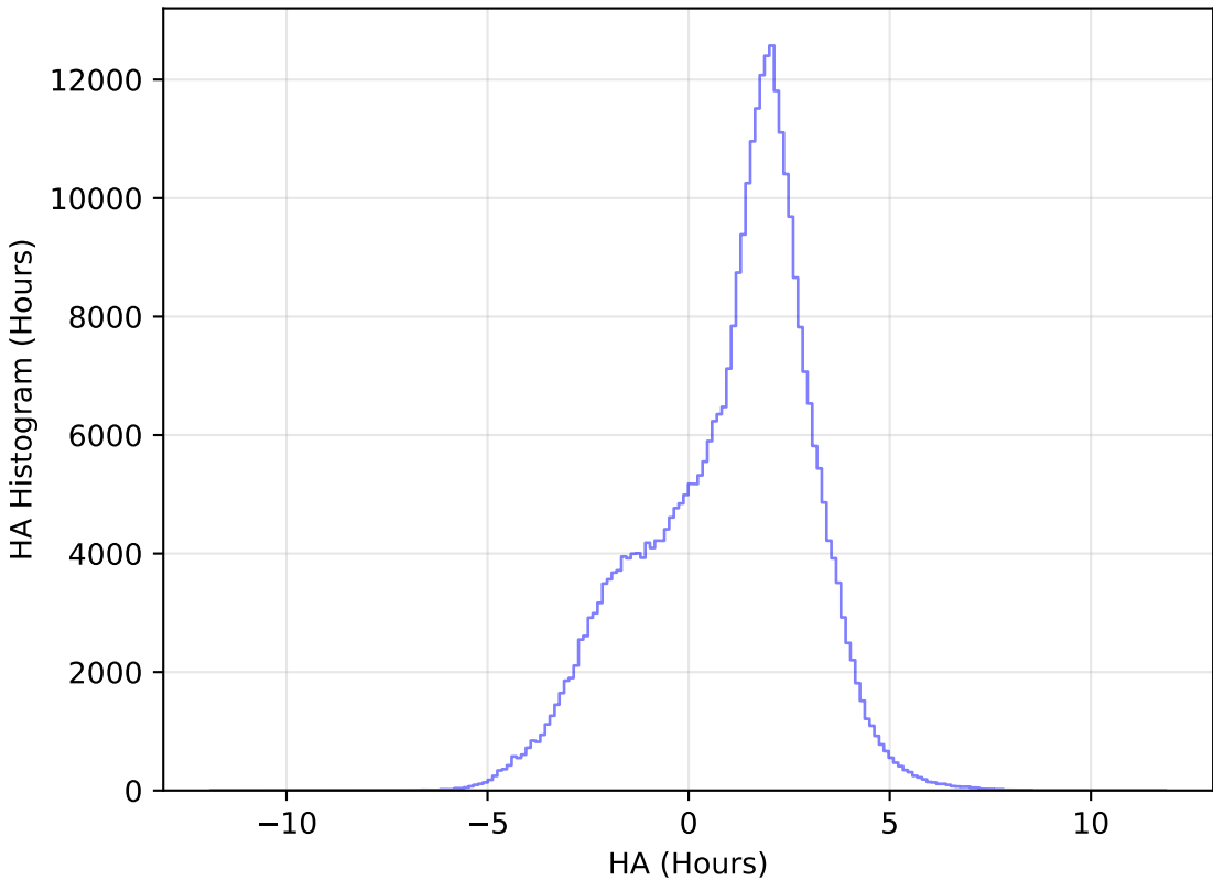
internal_u_expt45_nscale1.2v3.4_10yrs WFD y band: HA Histogram
