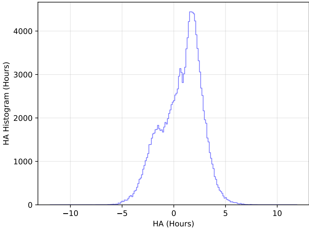
internal_u_expt45_nscale1.2v3.4_10yrs WFD u band: HA Histogram
