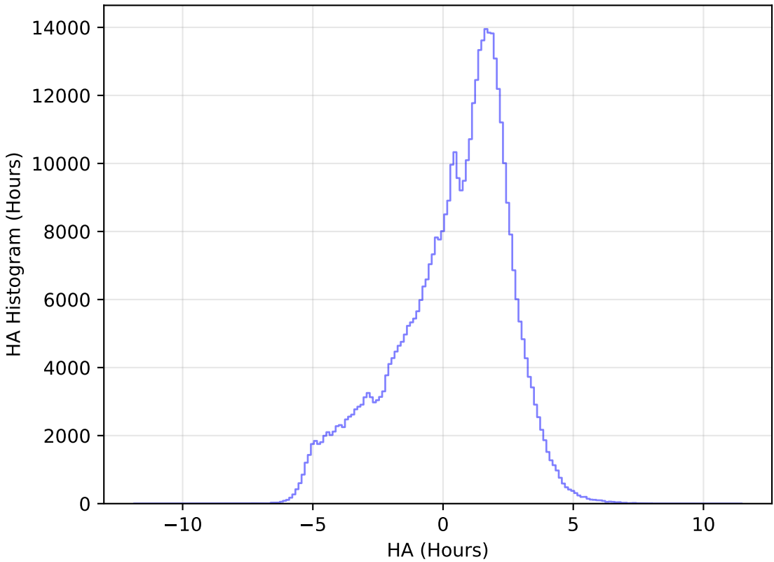
internal_u_expt45_nscale1.2v3.4_10yrs WFD r band: HA Histogram
