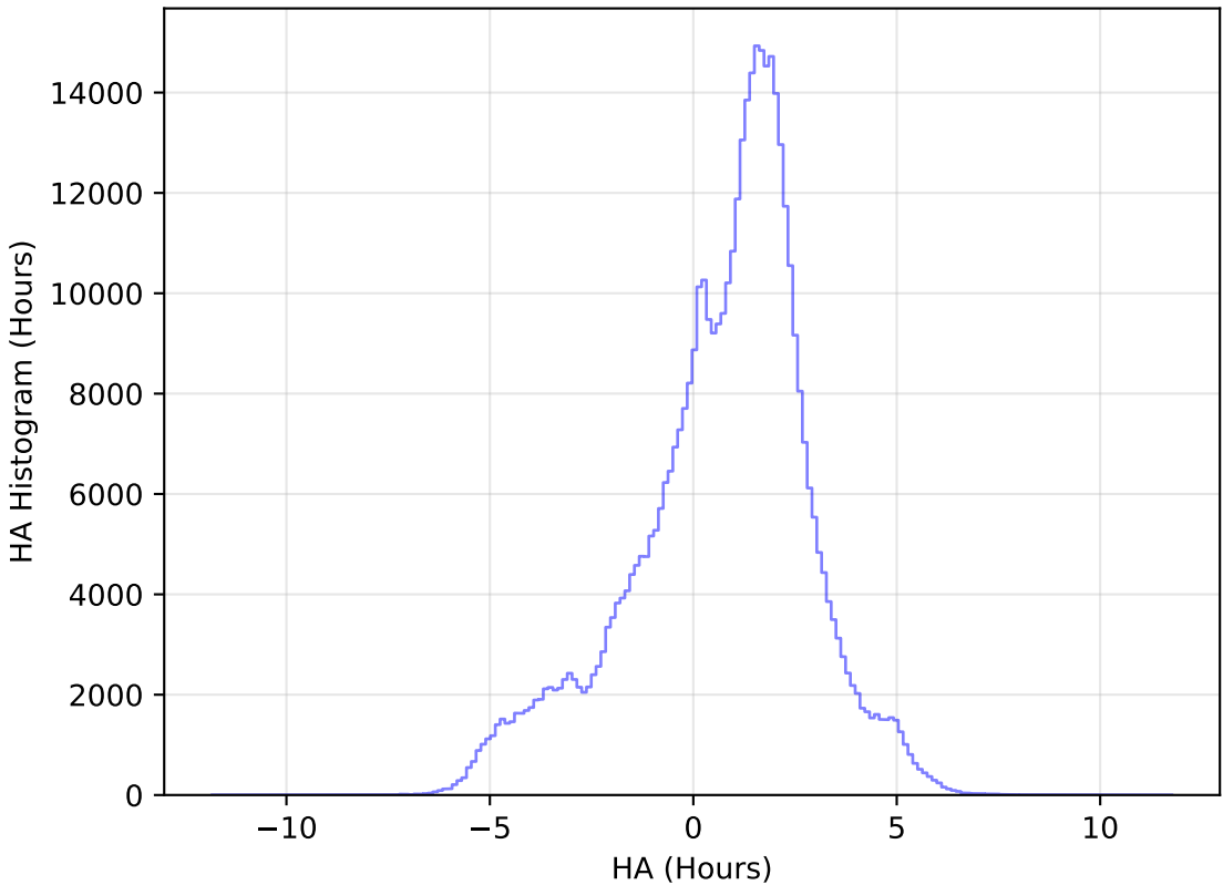
internal_u_expt45_nscale1.2v3.4_10yrs WFD i band: HA Histogram
