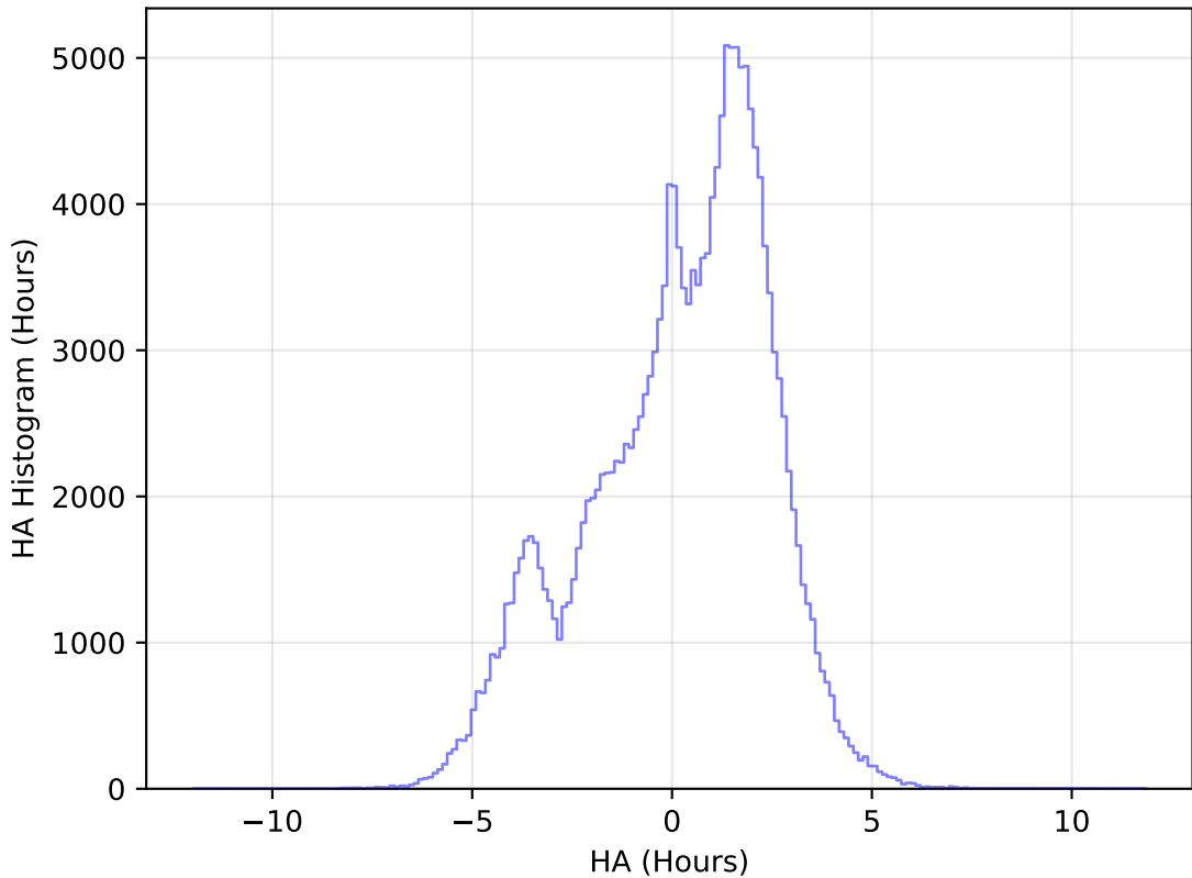
internal_u_expt45_nscale1.2v3.4_10yrs WFD g band: HA Histogram
