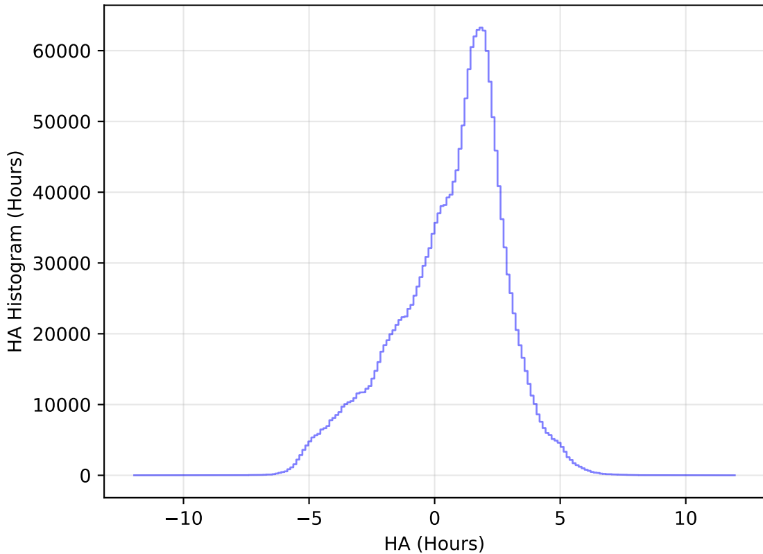
internal_u_expt45_nscale1.2v3.4_10yrs WFD all bands: HA Histogram
