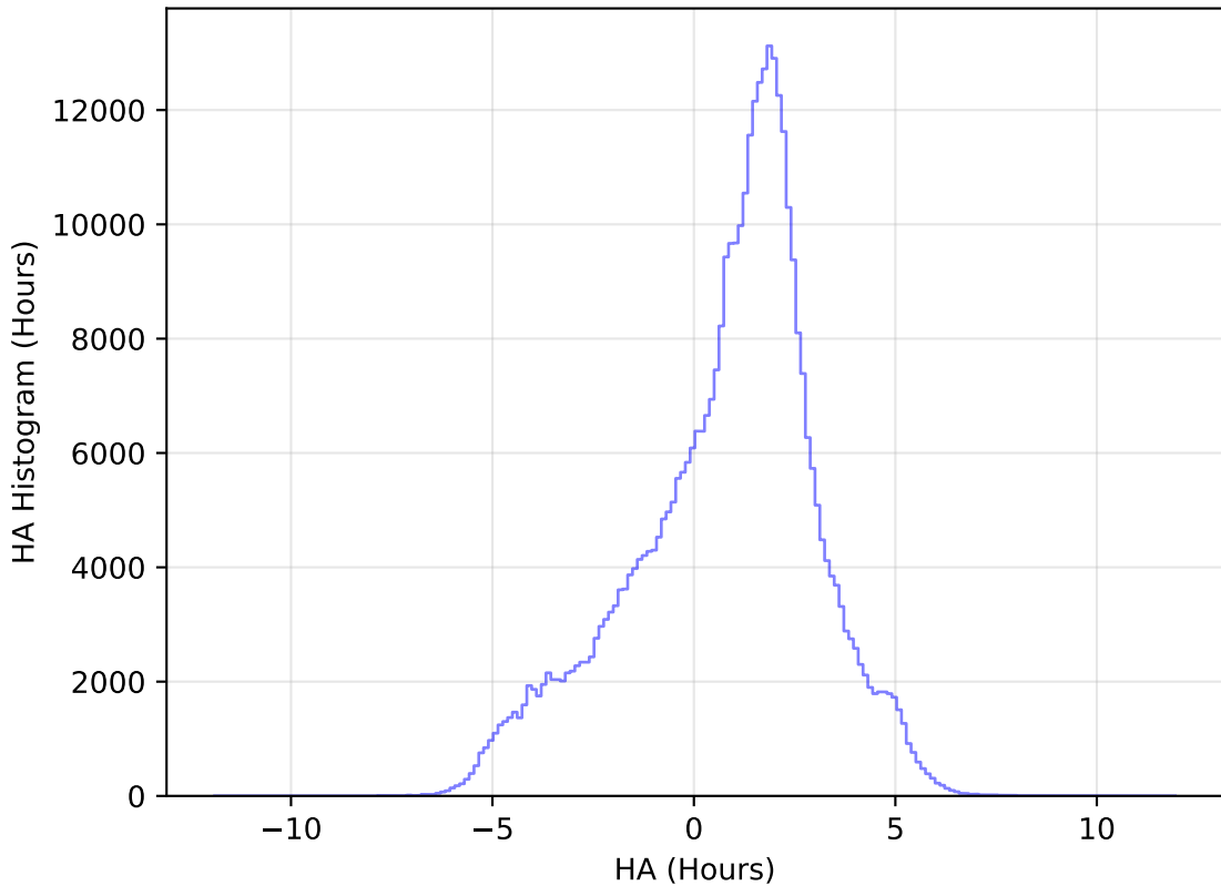
internal_u_expt45_nscale1.2v3.4_10yrs All sky z band: HA Histogram
