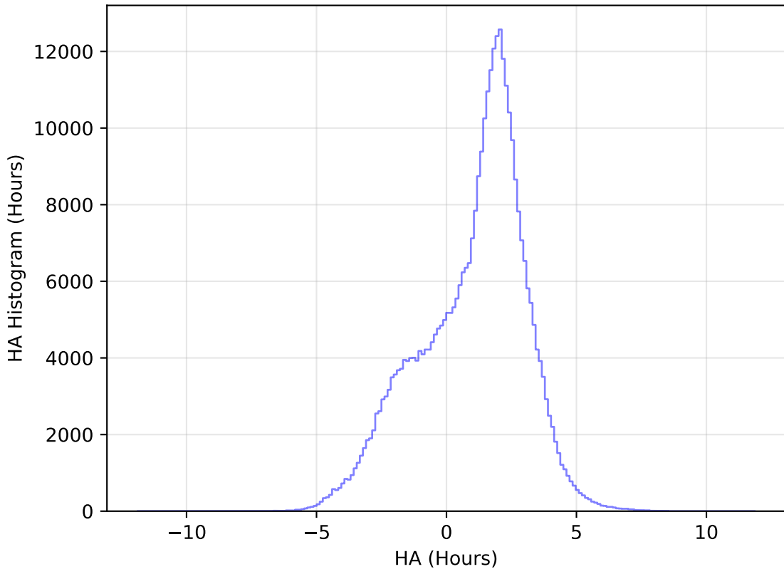
internal_u_expt45_nscale1.2v3.4_10yrs All sky y band: HA Histogram
